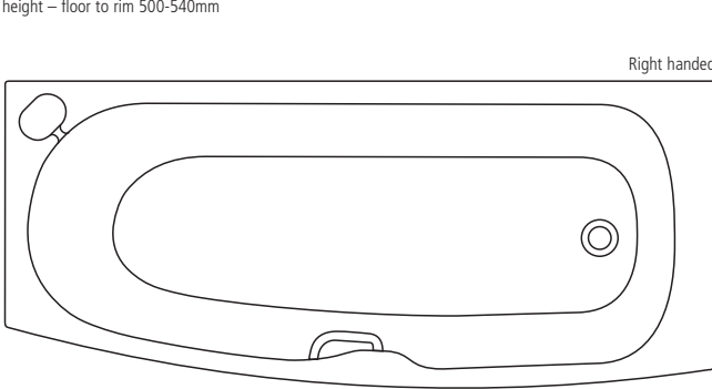
Studio 170 x 75cm Idealform shower right handed bath 1695 x 745mm height – floor to rim 500-540mm
