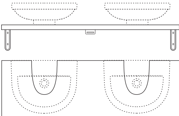
Washpoint 150cm Start furniture/vessel basin w1500 x d480mm
