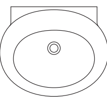
Kyomi 65cm basin w650 x d540mm
