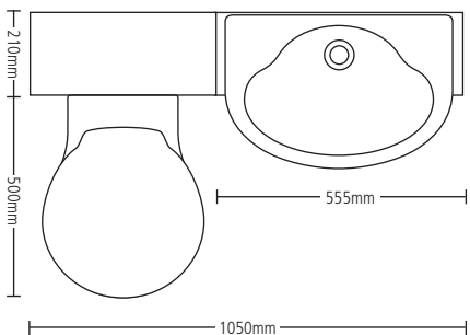
Space Illustration to show projection into the room of furniture, Space back-to-wall wc and basin
