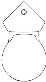
Space Corner close coupled wc suite w385 x d730mm seat position: conventional or turned 45° left or right
