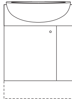
Space 60cm basin unit (one door) w600 x h800 x d210mm shown with optional plinth (h150mm) left and right hand options available
