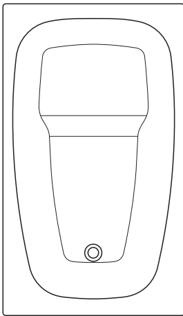
Space 120cm Idealform bath 1200 x 700mm height – floor to rim 510-550mm
