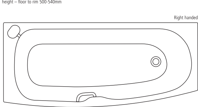
Studio 170 x 70cm Idealform spacemaker right handed bath 1695 x 695mm height – floor to rim 500-540mm
